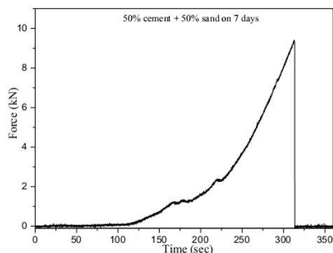
Fig. 7 Force Vs time for beam [17]
