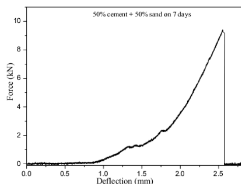
Fig. 9 Force Vs deflection for beam [17]
