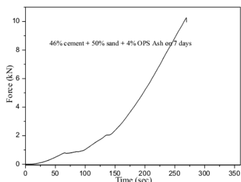
Fig. 8 Force Vs time for beam
