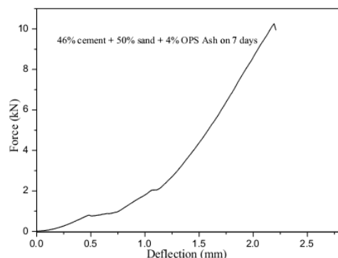
Fig. 10 Force Vs deflection for beam
