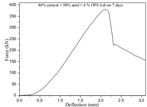
Fig. 4 Force Vs deflection for cubic specimen
