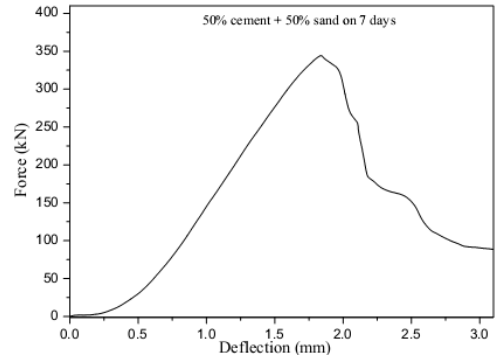
Fig. 3 Force Vs deflection for cubic specimen [17]
