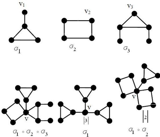
Fig. 2 Multiple coalescence G_1 \circ G_2 \circ G_3 , t -tuple coalescence \overset{|3|}{G_1} and coalescence of both G_1 \circ \overset{|2|}{G_2}
