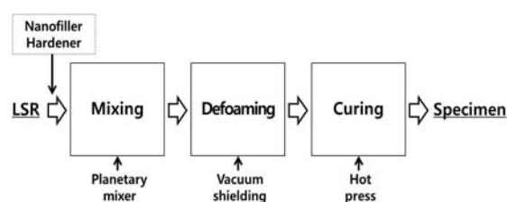
Fig. 1 Fabrication scheme of the specimens
