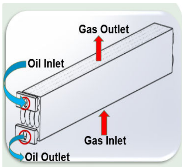
Fig. 1 Model of Finned-Tube Heat Exchanger
