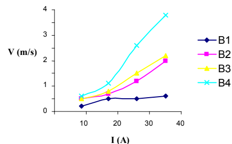
Fig. 4 Speeds of the arc movement for different values of blowing in the case of copper electrodes
