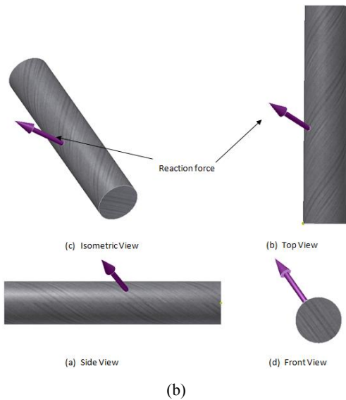
Fig. 2 (a) Reactions at the bottom roller due to bending force on top roller, (b) Bottom roller with 3-dimensional force pattern
