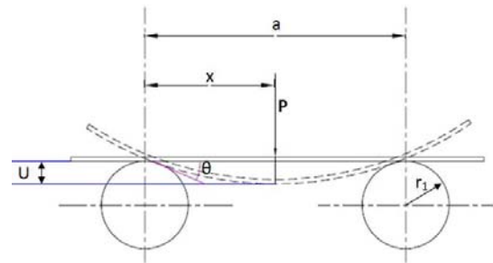
Fig. 3 Schematic of blank and roller arrangement for static bending
