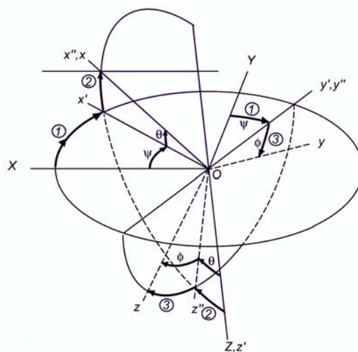
Fig. 2. Definition of Roll, Pitch and Yaw
