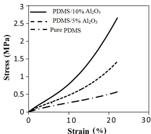
Fig. 1 Stress vs. strain behavior of PDMS /Al 2 O 3 composites compare to the pure PDMS elastomer
