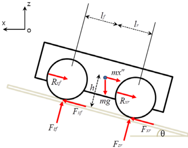
Fig. 1 The force acting on each wheel
