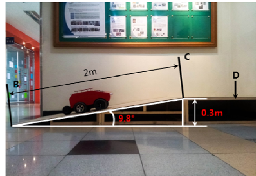
Fig. 3 Experiment in reference structures
