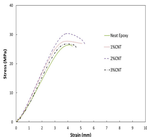
Fig. 5 Tensile diagrams of reference epoxy nanocomposites
