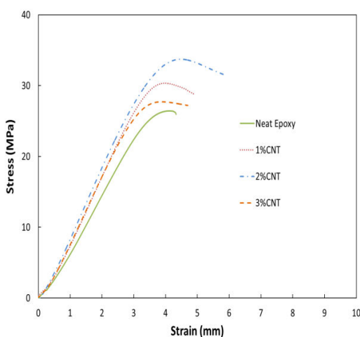
Fig. 6 Tensile diagrams of epoxy nanocomposites prepared with solvent
