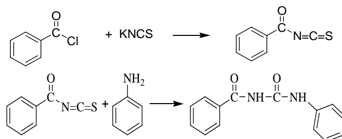
Fig. 2 Synthesises 1-phenyl -3-benzoyl-2- thiourea
