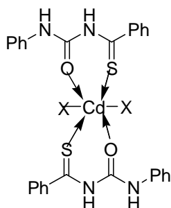
Fig. 1 Cadmium Complex Structure
