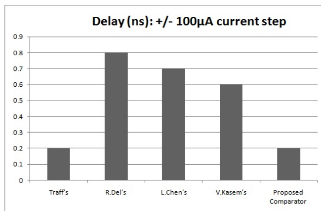
Fig. 7 Average Delay (ns): Response to +/- 100 \mu A Current Step
