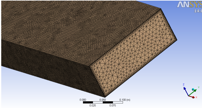
Fig. 3 Isometric view of the fluid domain meshing
