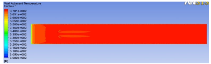
Fig. 12 Contours of wall adjacent temperature at Re 800
