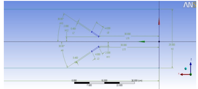
Fig. 1 Geometric model showing arrangement of blades (dimensions in cm)
