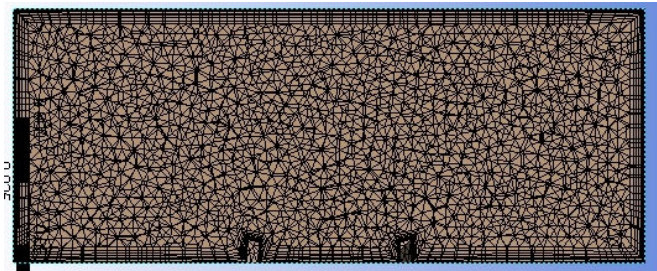
Fig. 4 Tetrahedral non uniform grid around the vortex generators (cross sectional view)
