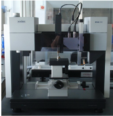
Fig. 1 Pendant drop DSA100 tensiometer (Krüss) was used to measure the IFT and ST
