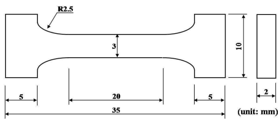
Fig. 2 Specifications of tensile specimens used in this study
