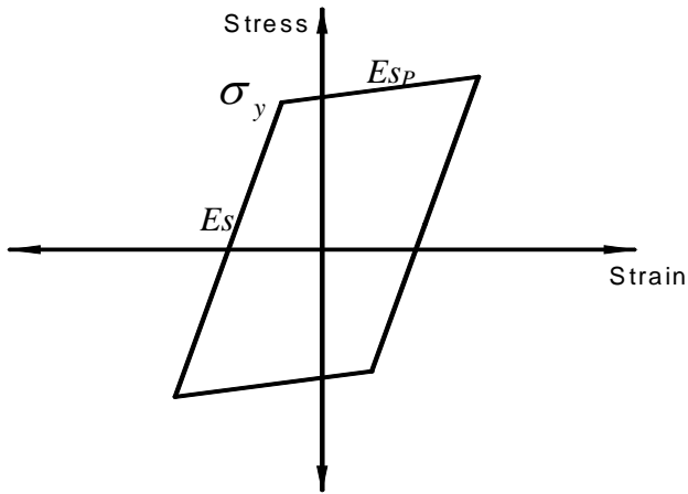
Fig. 3 Steel model
