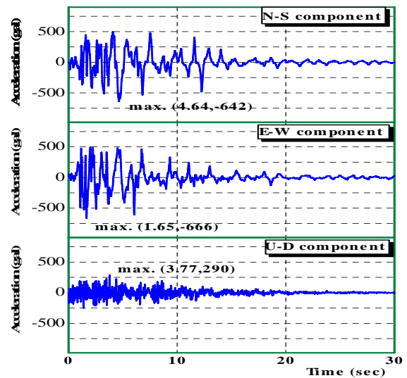
Fig. 4 Strong ground motion measured at JR Takatori
