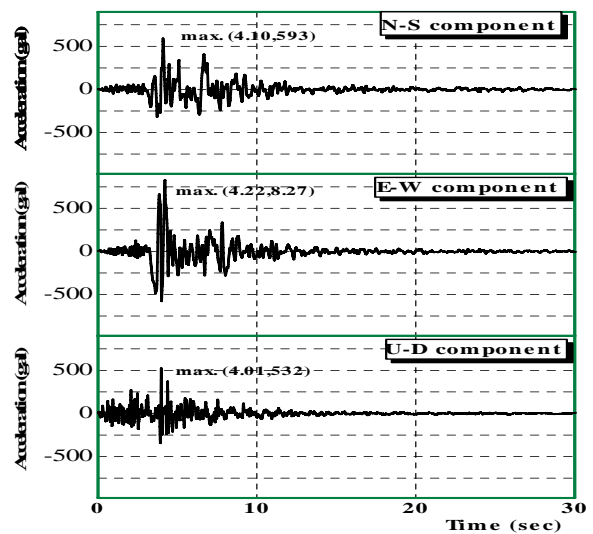
Fig. 5 Ground motion measured at Sylmar STA
