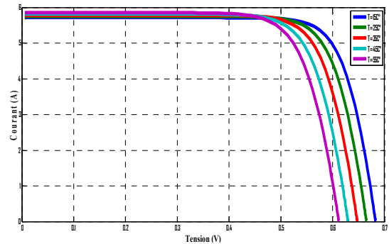
Fig. 6 Current variation with voltage at variable temperature
