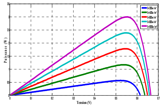
Fig. 5 Power variation with voltage at variable solar irradiance and fixed temperature
