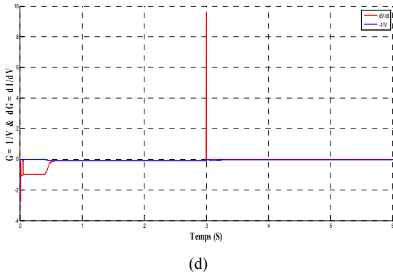
Fig. 12 Parameters behavior following the algorithm CI at negative jump of the irradiance G: (a) Voltage, (b) Current, (c) Power, (d) Conductance
