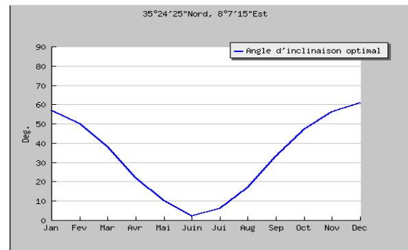
Fig. 16 Variation of the optimum angle of inclination of Ferkane municipality [17]
