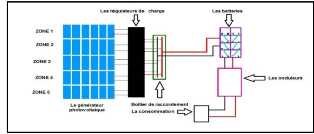
Fig. 18 Diagram of the photovoltaic array to supply Ferkene
