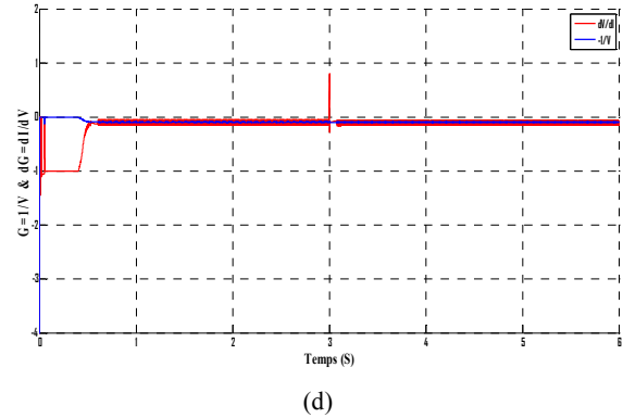
Fig. 13 Parameters behavior following the algorithm CI at positive jump of the irradiance G: (a) Voltage, (b) Current, (c) Power, (d) Conductance
