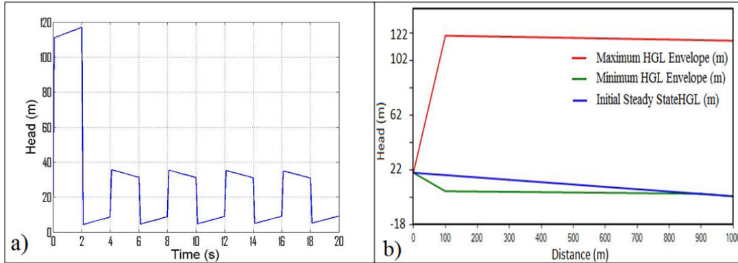
Fig. 7 Transients in pipeline system (Instant valve closure) (a) Head change versus time at the valve and (b) Hydraulic Grade Lines (with pressure relief valve protection)
