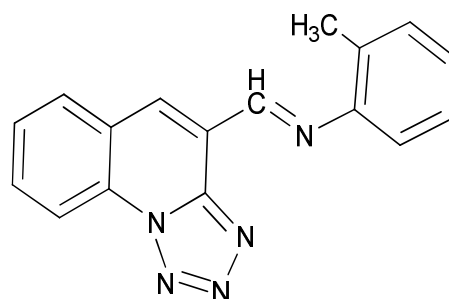
Fig. 1 (E)-2-methyl-N-(tetrazolo[1,5-a]quinolin-4-ylmethylene)aniline (QMA)
