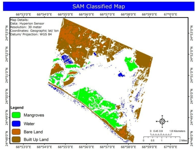
Fig. 2 Classified Study Area Map using SAM Technique
