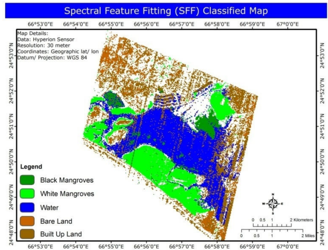
Fig. 3 Classified Study Area Map using SFF Technique
