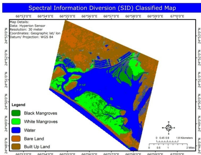
Fig. 4 Classified Study Area Map using SFF Technique
