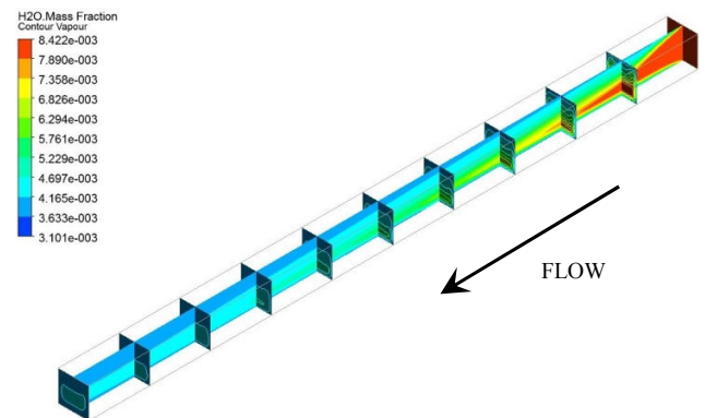
Fig. 3 Contours of water vapor mass fraction
