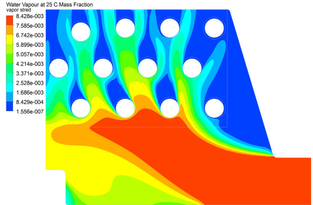
Fig. 8 Water vapor contours in middle plane
