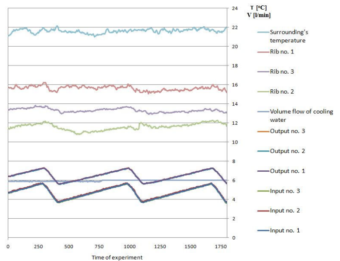
Fig. 6 Conditions during experiment (cut)
