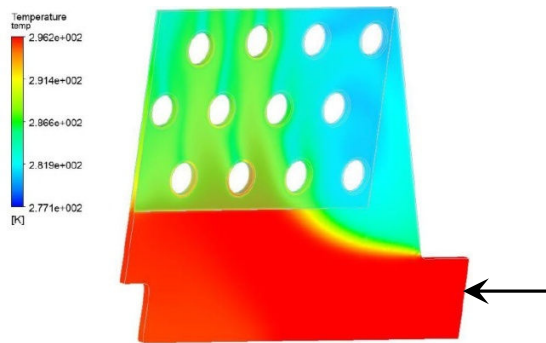
Fig. 7 Temperature field
