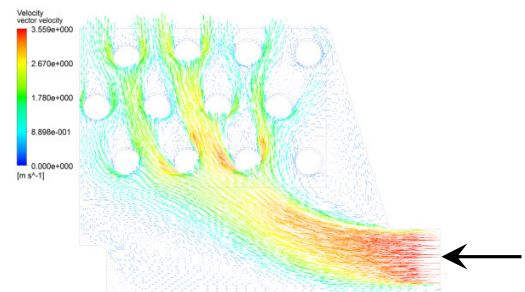
Fig. 9 Velocity field in middle plane
