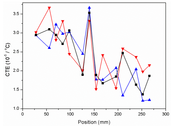
Fig. 10 Collection of results tested in three experiments
