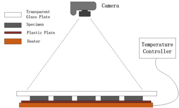
Fig. 7 Setup for test of CTE
