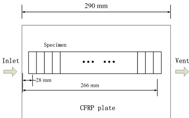
Fig. 6 Location of specimens
