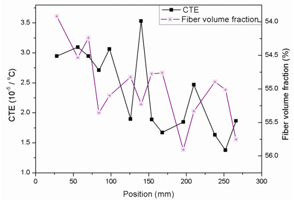
Fig. 9 Results of CTE and fiber volume fraction
