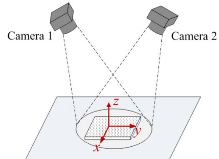
Fig. 2 Sketch of 3D-DIC method
