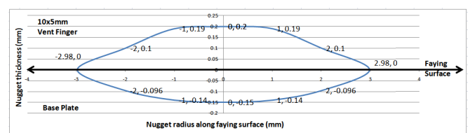
Fig. 8 Nugget geometry of 10x5mm vent finger
