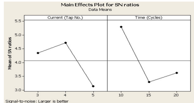
Fig. 2 Mean of S/N ratio in Taguchi analysis for 10 x 5mm
