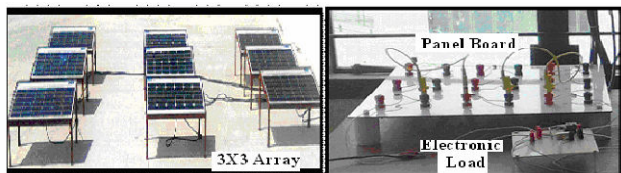
Fig. 6 Practical setup of a 3X3 array with Panel board and Electronic load
