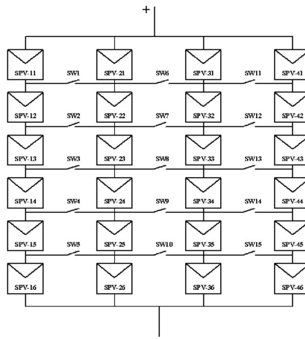
Fig. 7 Schematic of Electrical Reconfiguration of SPVA
