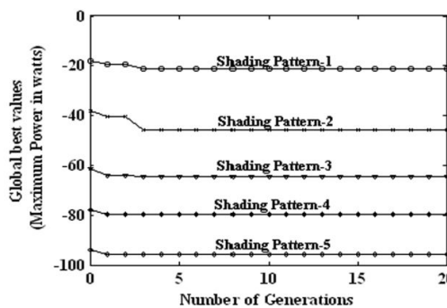
Fig. 8 The trend of convergence of PSO with the number of iterations for different shading patterns
