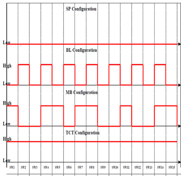
Fig. 9 Pulse pattern given to switches for reconfiguration
