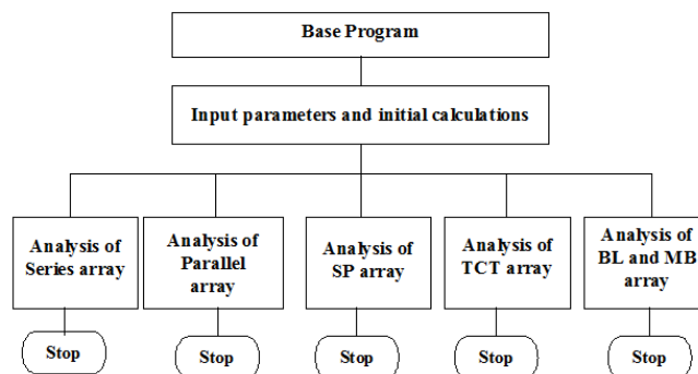
Fig. 5 Architecture of the developed software
