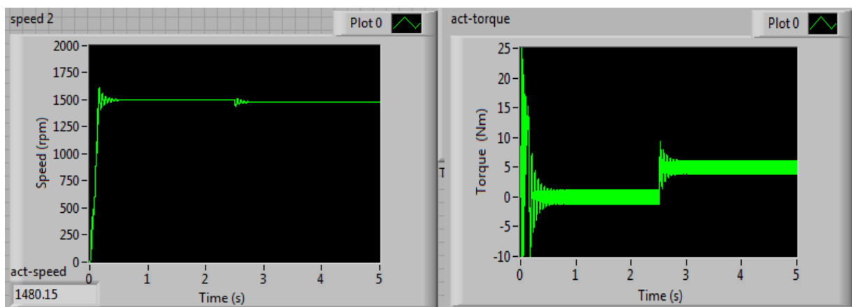
Fig. 3 Speed and torque waveforms of induction motor
