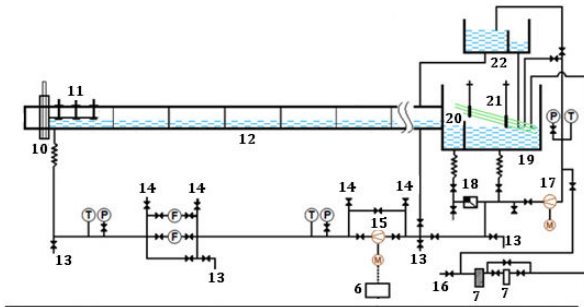
Fig. 8 Schematic of water supply cycle (MFL-TMU)
