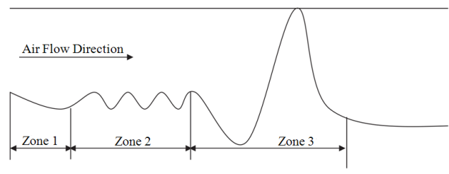
Fig. 1 Schematic of slug flow with three regions [11]
