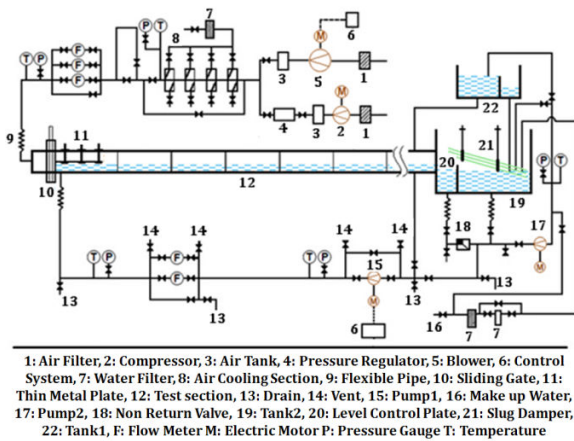
Fig. 3 Schematic of the experimental apparatus at the MFL-TMU
