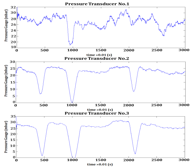
Fig. 16 Pressure behavior at a liquid holdup of 0.50, U_{sl}=0.33\text{m/s} , U_{sg}=4.47\text{m/s} , Test No. 8
