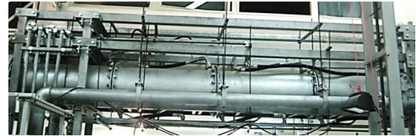
Fig. 5 Picture of air cooling line (MFL-TMU)
