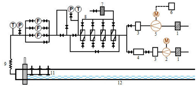
Fig. 4 Schematic of the air supply loop (MFL-TMU)
