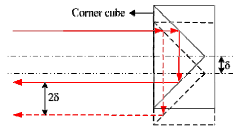
Fig. 3 Sketch of the increasing resolution
