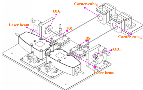
Fig. 1 Sketch of the 2-D optical measurement system
