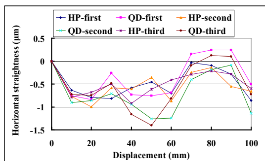
Fig. 4 Verification results of horizontal straightness
