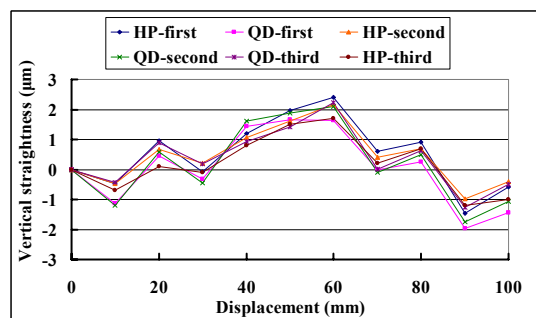
Fig. 5 Verification results of vertical straightness
