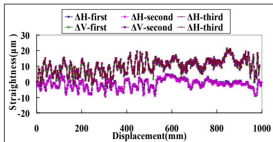
Fig. 6 Results of horizontal and vertical straightness measurements
