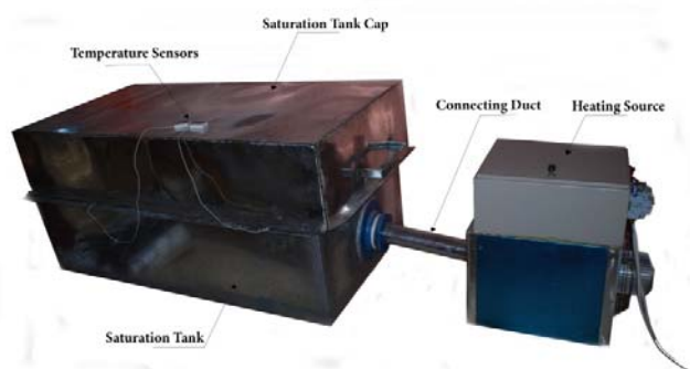
Fig. 2 Saturation-Drying System
