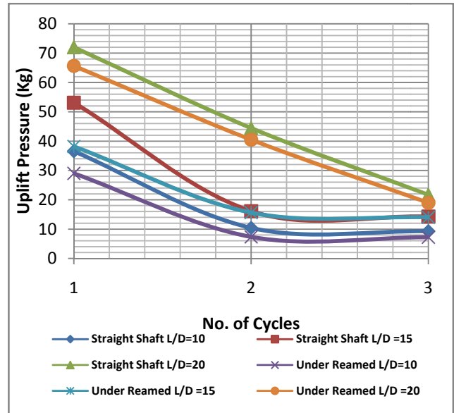
Fig. 5 Pile Uplift Pressure Reduction through Wetting-Drying Cycles
