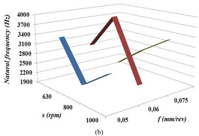
Fig. 6 Relationship between natural frequency, spindle speed (s) and feed rate (f) in turning of AA2024 with: (a) standard cutting tool and (b) cutting tool with holes in toolholder
