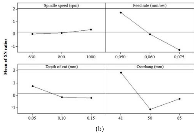
Fig. 5 Main effect plots for S/N ratios of R_a for: (a) standard cutting tool and (b) cutting tool with holes in toolholder
