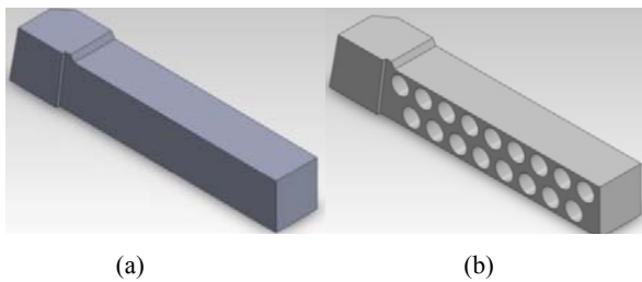
Fig. 1 3D- model of the cutting tools in SolidWorks: (a) standard cutting tool; (b) cutting tool with horizontal holes arranged in a chess-board pattern (Ø 10 mm)
