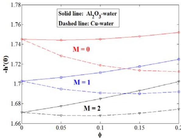
Fig. 12 Variation of the local Sherwood number -h'(0) with \phi for different values of M , when S = 1, Pr = 6.2, A^* = B^* = 0.05, Sc = 1 in case of Al_2O_3 –water and Cu –water nanofluids
