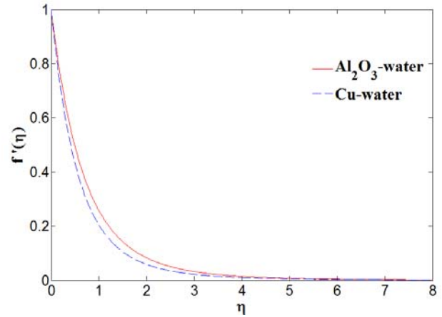
Fig. 2 Velocity distribution f'(\eta) of Al_2O_3 -water and Cu -water nanofluids, when \phi = 0.2 , M = S = 1 , Pr = 6.2 , A^* = B^* = 0.05 , Sc = 1
