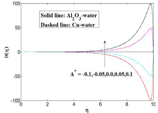
Fig. 6 Effects of A^* on the temperature distribution \theta(\eta) , when \phi = 0.2 , M = S = 1 , Pr = 6.2 , B^* = 0.05 , Sc = 1 in case of Al_2O_3 –water and Cu –water nanofluids
