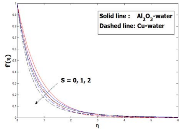
Fig. 3 Effects of S on the velocity distribution f'(\eta) , when \phi = 0.2 , M = 1 , Pr = 6.2 , A^* = B^* = 0.05 , Sc = 1 in case of Al_2O_3 -water and Cu -water nanofluids
