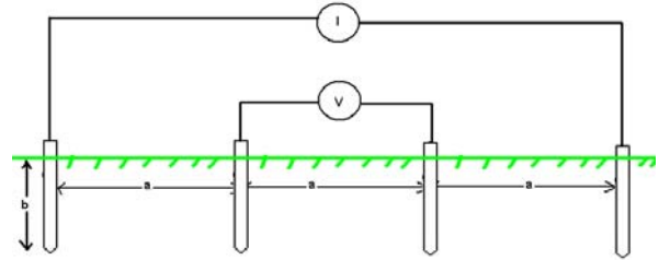
Fig. 2 Wenner Method for Soil Resistivity Test
