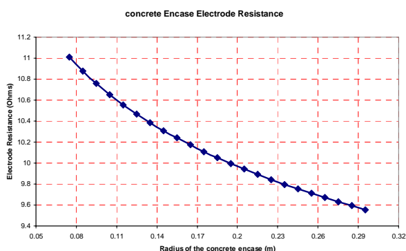
Fig. 4 Electrode Resistance under different concrete encase radius
