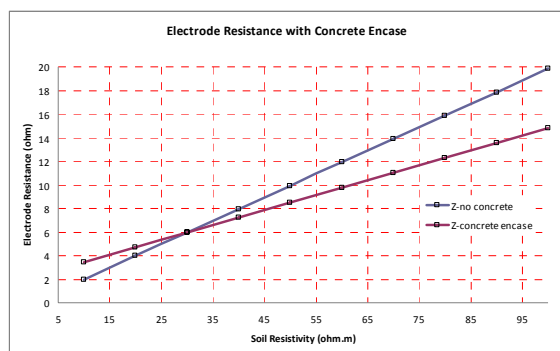
Fig. 3 Electrode resistance under concrete encasement
