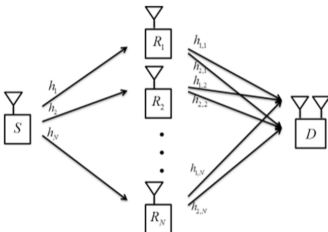
Fig. 1 Dual-hop cooperative wireless system
