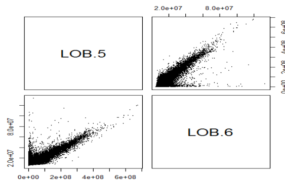
Fig. 2 Pairs plot of the simulated loss data for LOBs 5 and 6.
