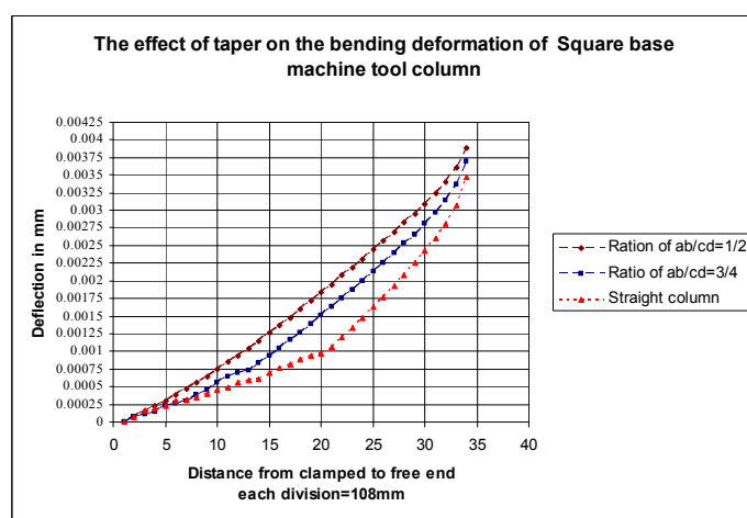
Fig. 6 The effect of taper on the bending deformation of square base machine tool column
