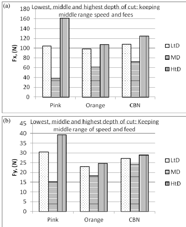
Fig. 6 Effect due to depth of cut; (a) normal force (b) tangential force
