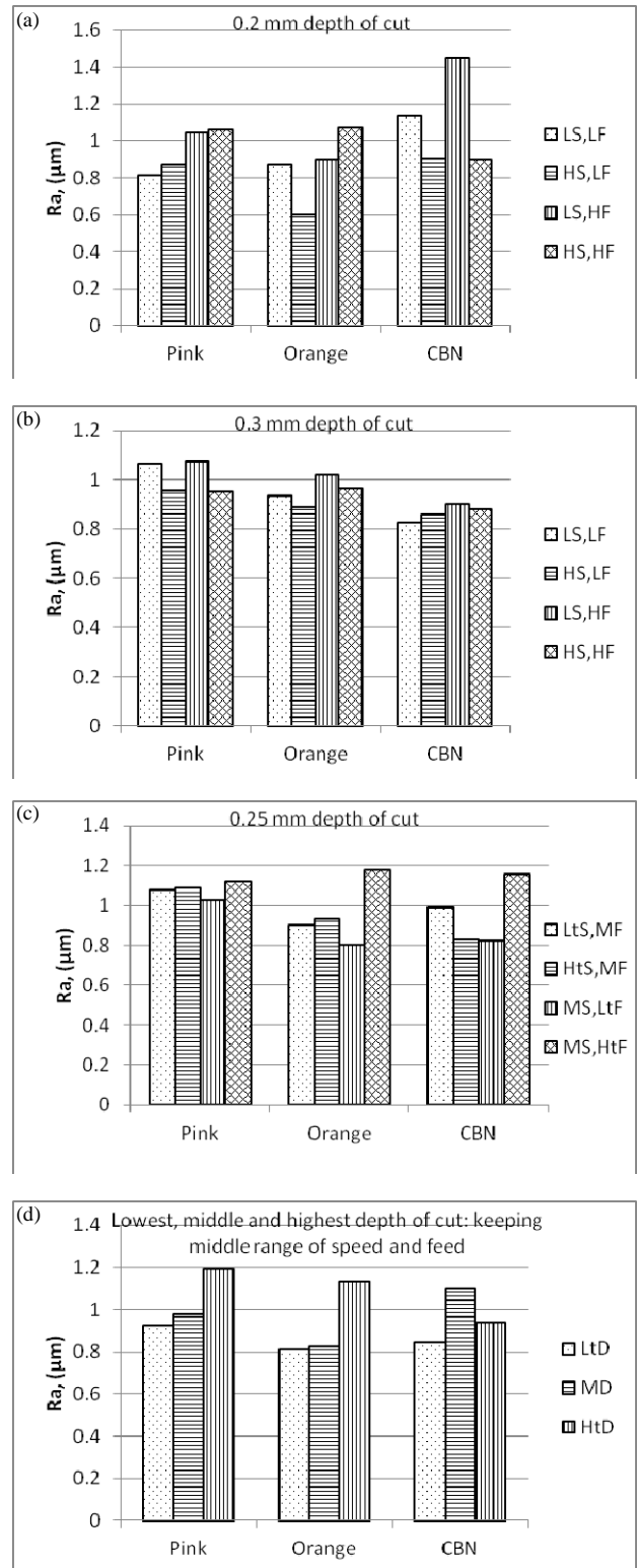
Fig. 7 Parametric influence on surface finish compared between P- \text{Al}_2\text{O}_3 and O- \text{Al}_2\text{O}_3 , and c-BN grinding wheels (a) 0.2 mm depth of cut (b) 0.3mm depth of cut (c) 0.25 mm depth of cut (d) lowest, highest and middle depth of cut
