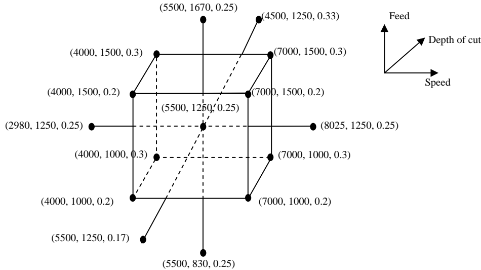
Fig. 2 Experimental design space with selected parameters
