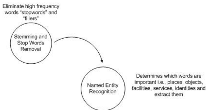
Fig. 4 Framework Stage 2
