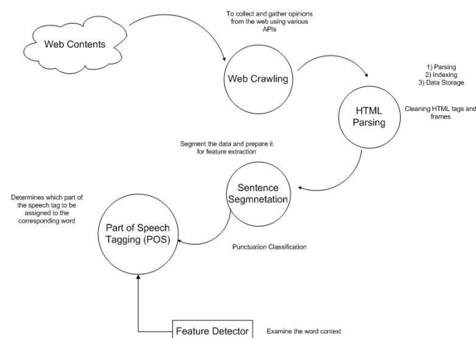
Fig. 1 Framework Stage 1
