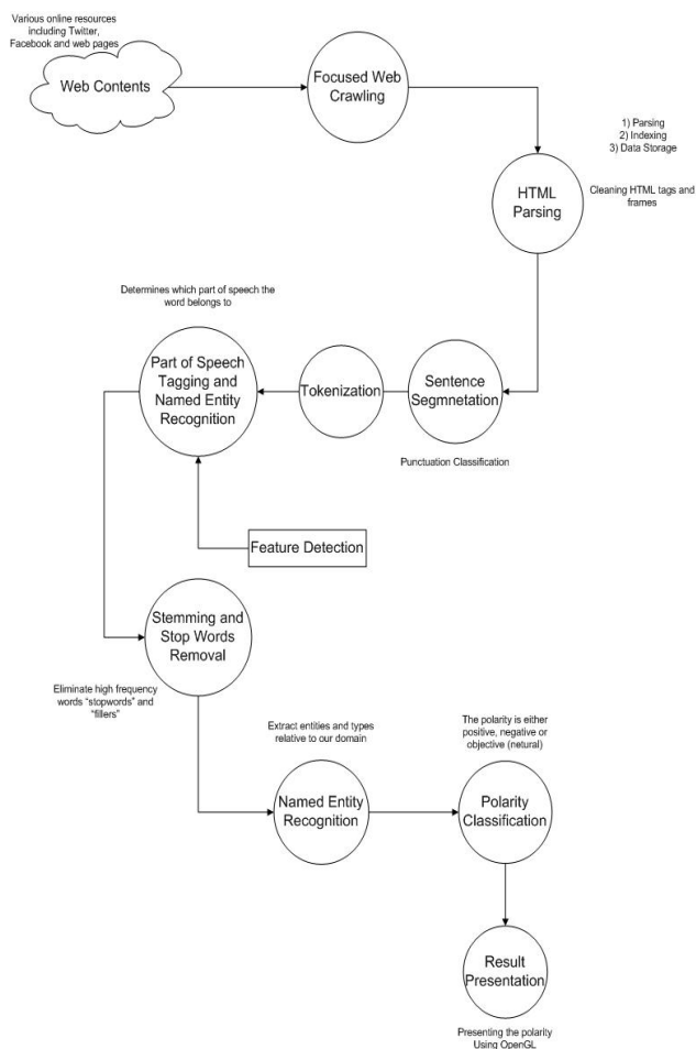
Fig. 8 Overall Framework
