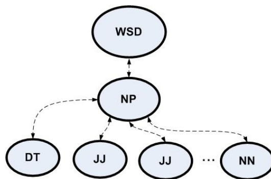
Fig. 5 WSD Tree
