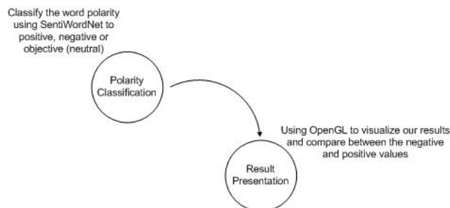
Fig. 6 Framework Stage 3
