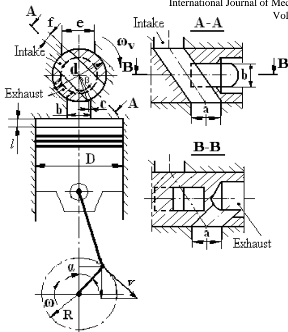
Fig. 1 Gas intake and exhaust in rotating valve
