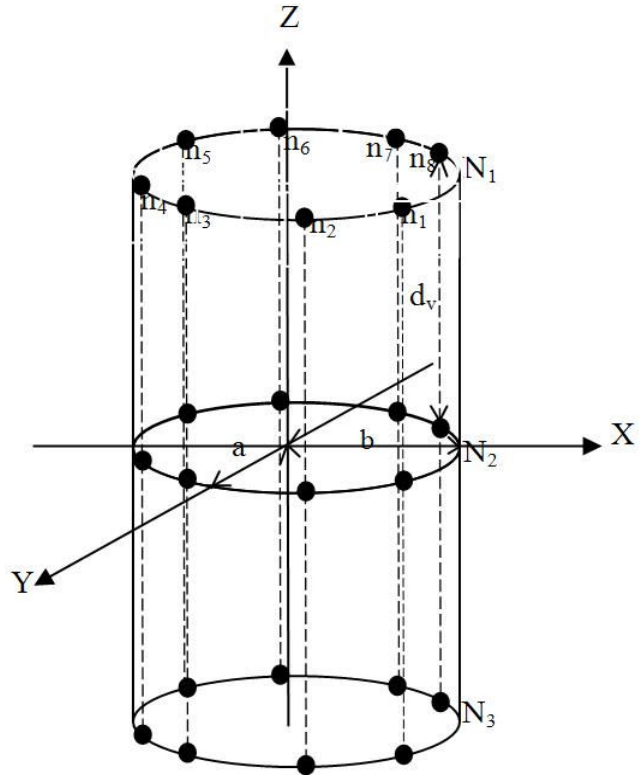
Fig. 1 Elliptical cylindrical array (ECA) structure
