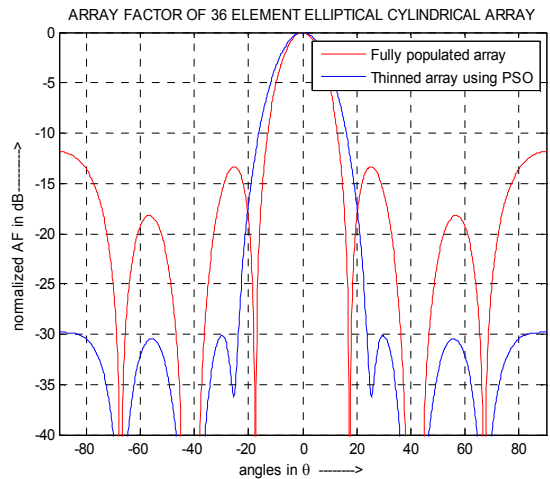
Fig. 6 Normalized absolute power patterns in dB for fully populated array and thinned array with fixed inter-element spacing d=0.7\lambda .
