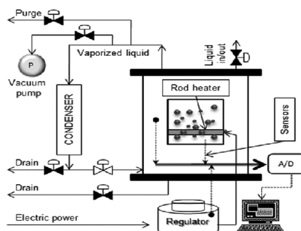
Fig. 1 The schema of test equipment
