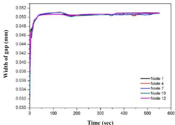
Fig. 8 The variations of gap width in the rod during transient at T03 zone
