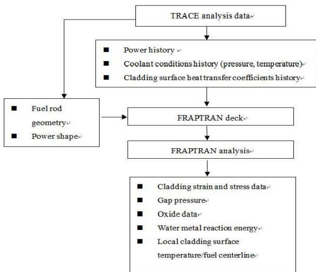
Fig. 2 The flowchart of combining TRACE and FRAPTRAN
