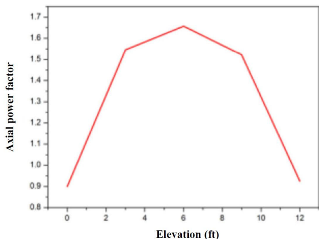
Fig. 6 The axial power shape data of TRACE
