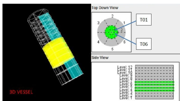
Fig. 4 The TRACE vessel structure model of Maanshan NPP
