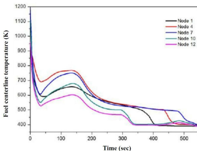
Fig. 11 The fuel centerline temperatures at T01 zone
