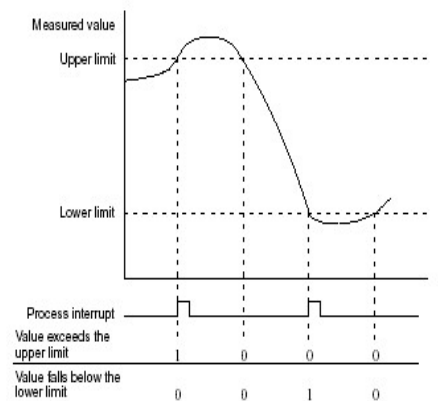
Fig. 5 Conditions interrupting for analog signal
