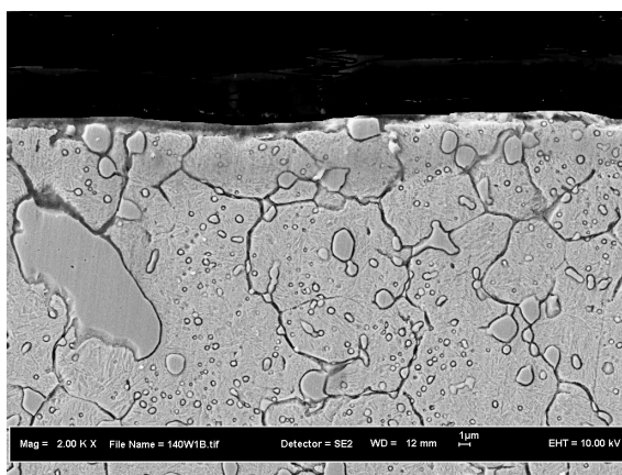
Fig. 2 Thin white layers (1µm) were observed in single pass cutting
