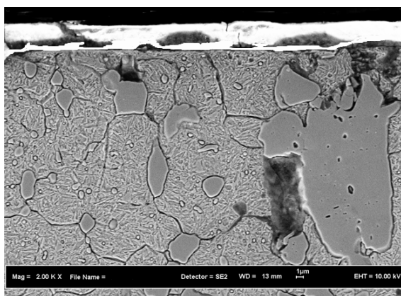
Fig. 3 Thicker white layers (3µm) can be observed in 20 pass cutting
