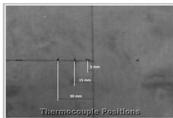
Fig. 2 Thermocouple positions
