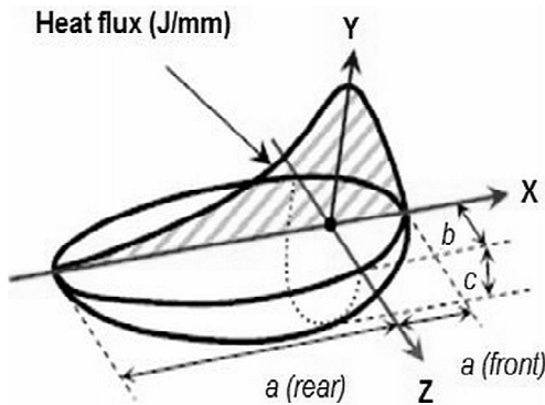
Fig. 5 Heat Input Model
