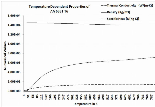
Fig. 3 Temperature dependent properties of AA6351 T6
