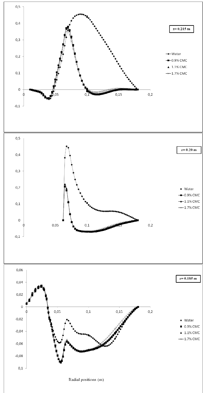
Fig. 8 Radial profiles of axial velocity (m / s)
