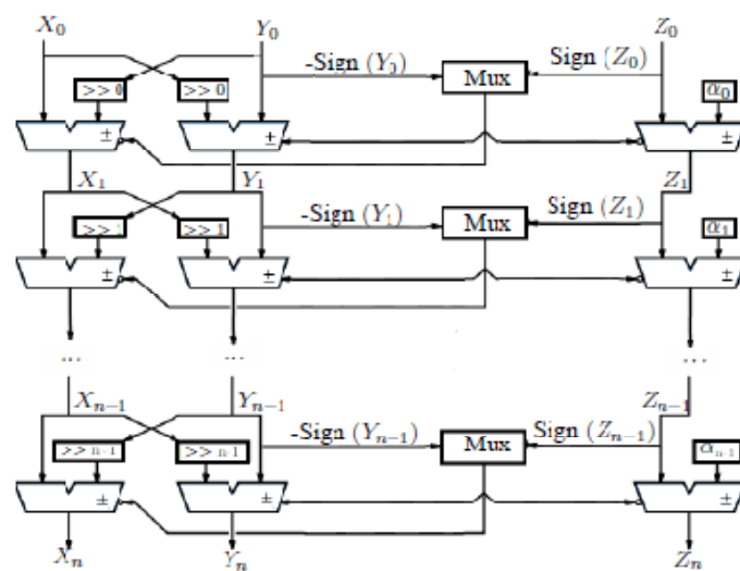
Fig. 2 Unfolded Pipelined CORDIC Architecture
