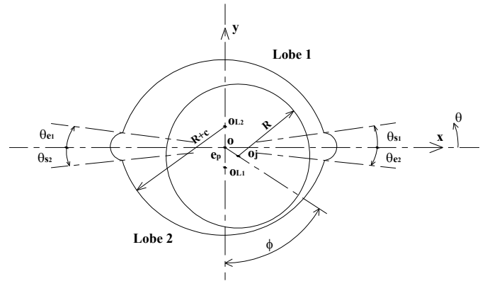
Fig. 1 Journal Bearing Configurations
