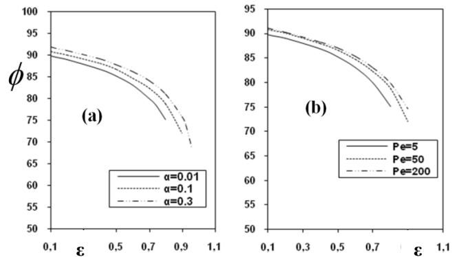
Fig. 3 \phi versus \epsilon . (a) for various values of \alpha (b) for various values of Pe
