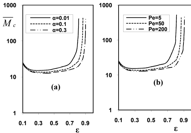
Fig. 5 \bar{M}_c versus \epsilon . (a) for various values of \alpha (b) for various values of Pe
