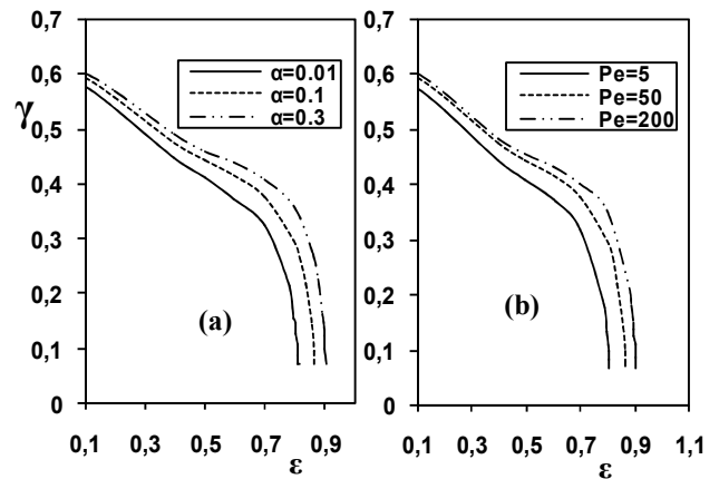
Fig. 6 \gamma versus \epsilon . (a) for various values of \alpha (b) for various values of Pe
