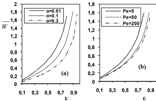
Fig. 4 \bar{W} versus \epsilon . (a) for various values of \alpha (b) for various values of Pe
