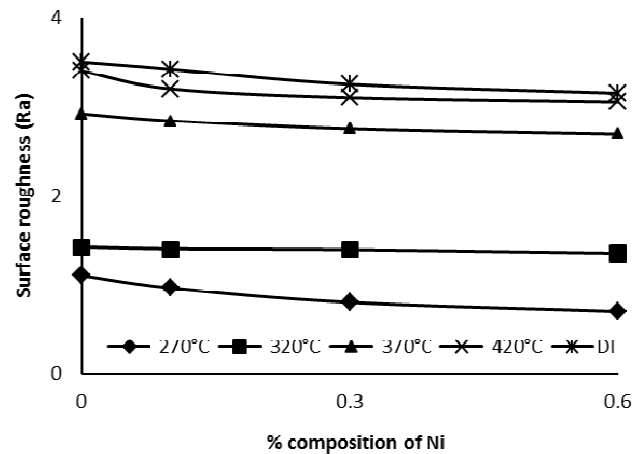
Fig. 6 Surface Roughness (Ra(μ)) of DI and ADI samples
