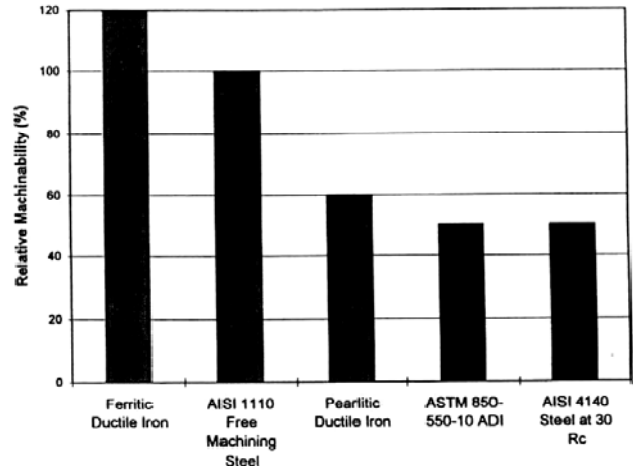
Fig. 1 Relative machinability of several ferrous materials
