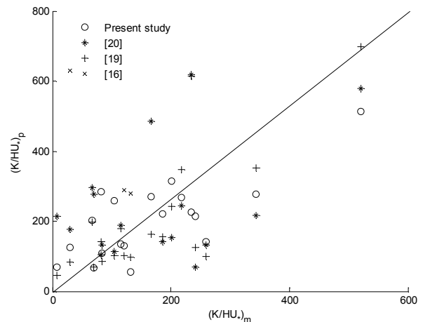
Fig. 4 Measured vs. predicted K_f/HU_* (verification dataset)
