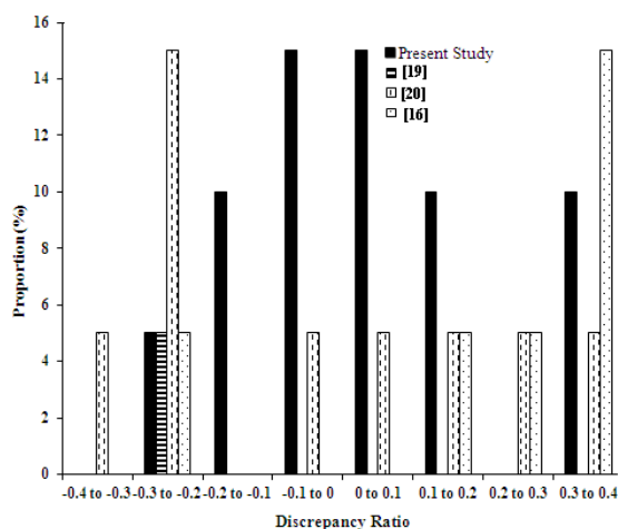
Fig. 5 DR values by models (verification dataset)
