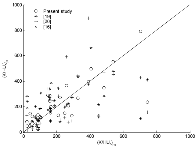
Fig. 3 Measured vs. predicted K_f/HU_* (derivation dataset)
