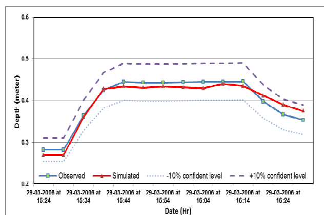
Fig. 8 Verified event on 29 March 2006
