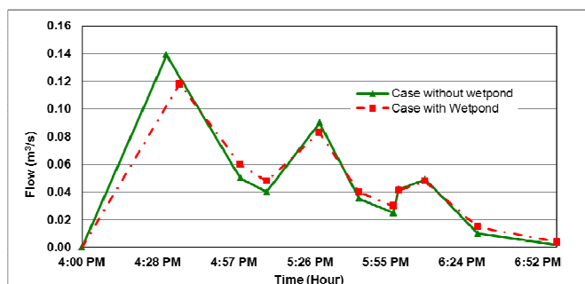
Fig. 9 Comparison case with and without constructed wet pond for calibrated event on 26 February 06
