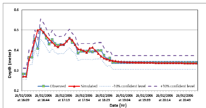
Fig. 6 Calibrated event on 26 February 2006
