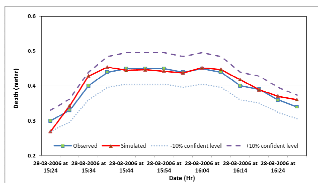
Fig. 7 Calibrated event on 28 March 2006
