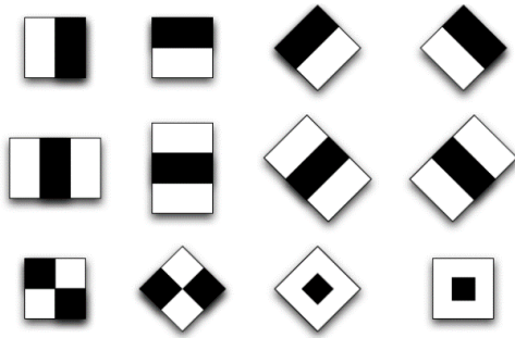
Fig. 1 Basic types of Haar features
